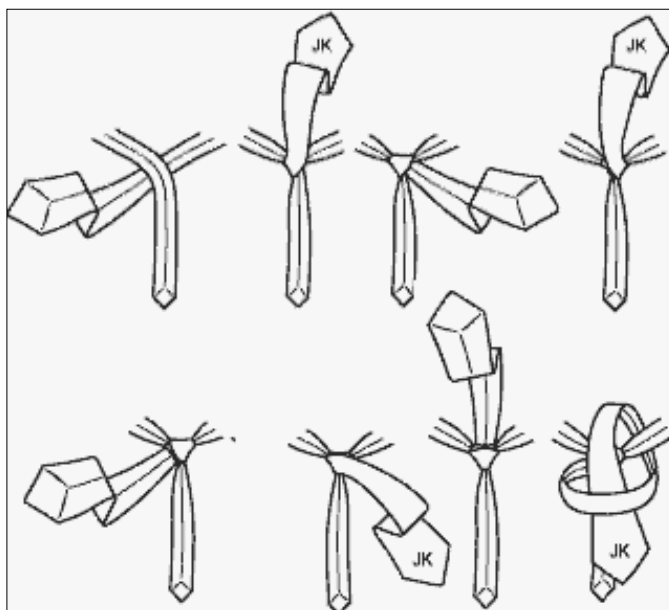
Plattsburgh Knoten
