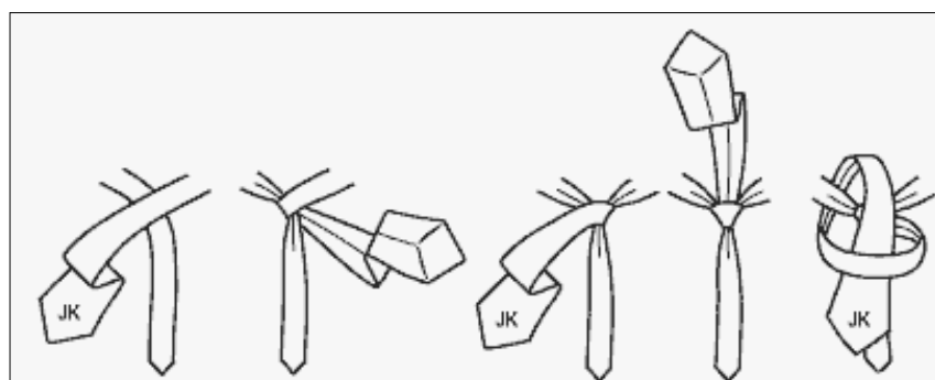
Four-in-Hand Knoten
